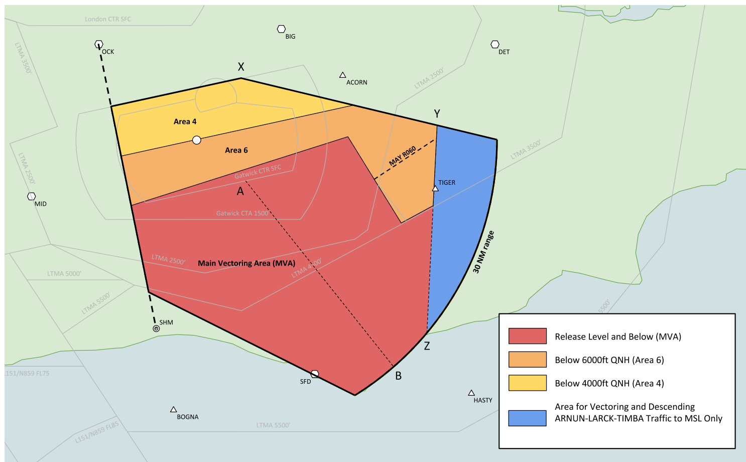
Figure 8 – Gatwick RMA – Westerly Operations
