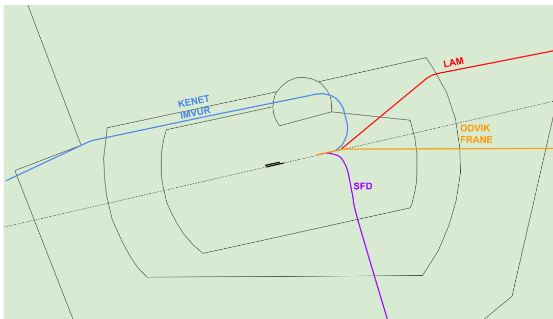
Figure 6 – Illustration of SID Tracks – Easterly Operations
