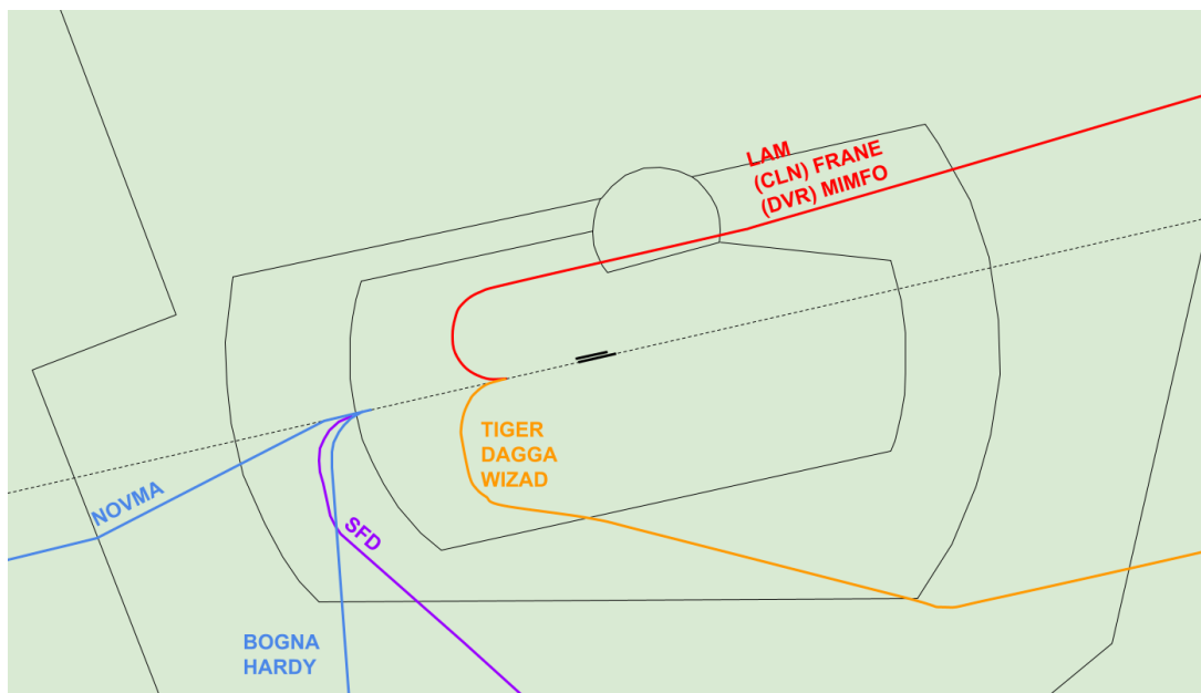
Figure 5 – Illustration of SID Tracks – Westerly Operations
