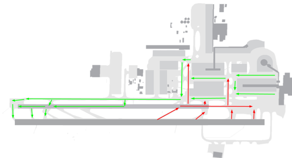
Figure 4 – Suggested Taxi Routings – Easterly Operations
