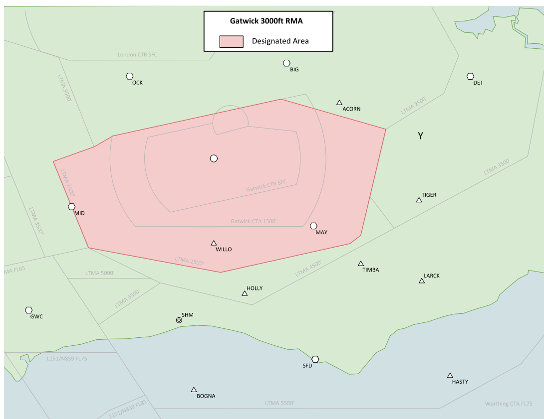
Figure 7 – Gatwick RMA (3000 ft)
