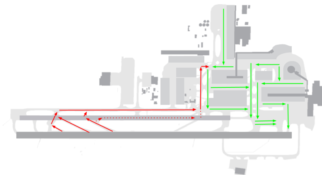
Figure 3 – Suggested Taxi Routings – Westerly Operations
