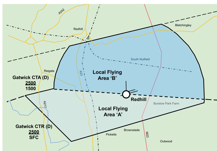
Figure 10 – Redhill Local Flying Area (LFA)
